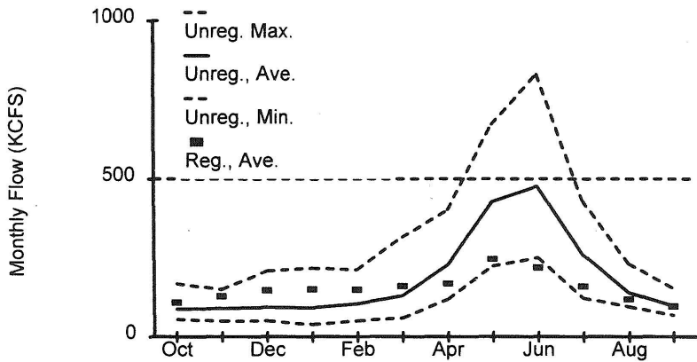
Figure 5B.3. Long-term unregulated (1928-89; BPA 1993) and regulated (1991-94) monthly Columbia R. flows at The Dalles.
